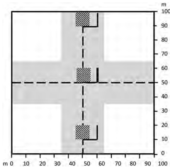
Fig. 3. Design of 1 ha (100 m \times 100 m) experimental sites showing the central and perpendicular transects (dashed lines), 10 m \times 10 m plots (hatched), 10m transects (black lines), and area sampled for large trees 2 \times 30 m \times 100 m = 0.51 ha (grey shaded area). Different biomass components were sampled in different parts of the site.
