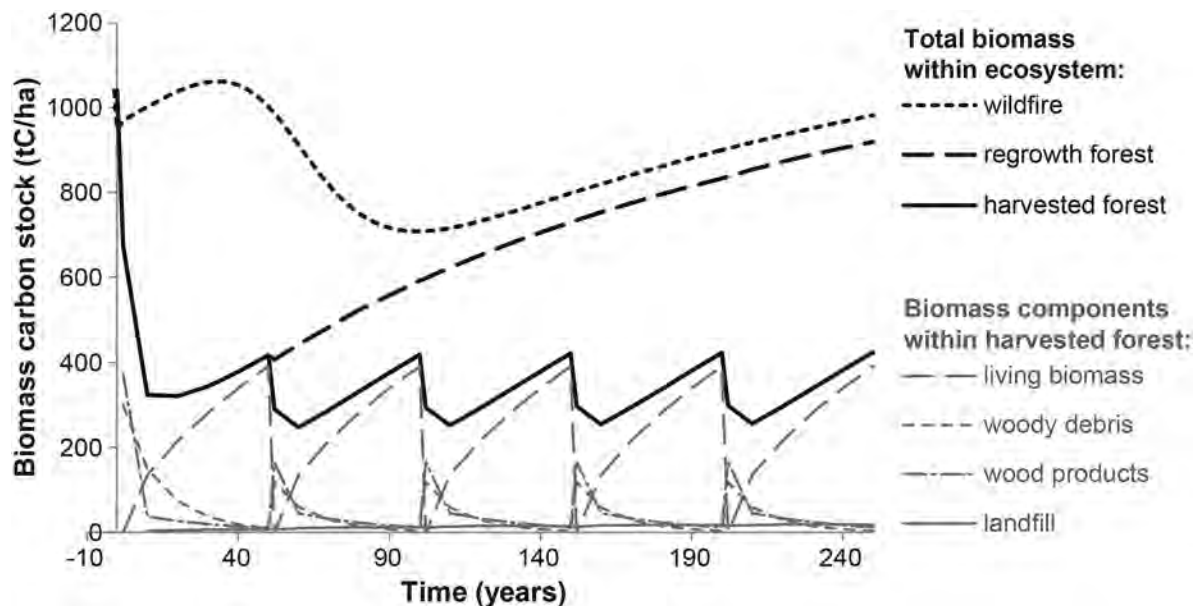
Fig. 10. Changes in total biomass carbon stock of the ecosystem over time under three scenarios (shown as black lines) from an initial stock of a native forest: (1) wildfire that occurred at time 0 years and then the forest regenerated and dead biomass decomposed over time, (2) regrowth forest after logging once and regeneration, and (3) harvested forest under a regime of repeated logging rotations consisting of clearcutting and slash burning on a 50 year cycle (Timber Industry Strategy State of Victoria, DPI 2009). The carbon stock within the harvested forest is separated into biomass components (shown as grey lines): (1) living biomass, (2) dead and downed woody debris, (3) wood products, and (4) landfill. These biomass components constitute part of the harvested forest system but are not all located at the same site; living biomass and dead and downed woody debris occur at the forest site, but wood products and landfill occur in different locations. The proportions allocated to each of these components and their rates of stock change are derived from the data in Fig. 8 and Appendix E: Table E1. Sustainable production is assumed over the course of the rotations.
